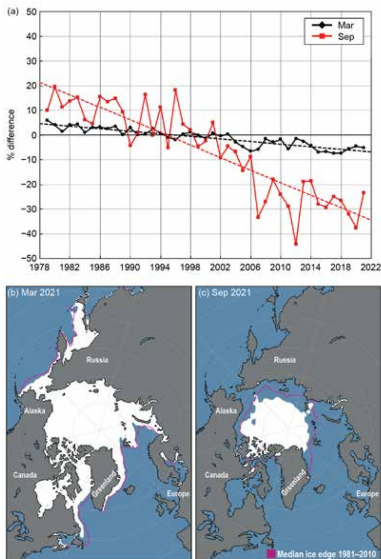
Fig. 5.7. (a) Monthly sea ice extent anomalies (solid lines) and linear trend lines (dashed lines) for Mar (black) and Sep (red) from 1979 to 2021. The anomalies are relative to the 1981–2010 average for each month. (b) Mar 2021 and (c) Sep 2021 monthly average sea ice extent; the median extent for 1981–2010 is shown by the magenta contour.
