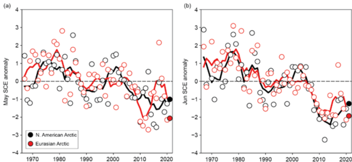
Fig. 5.19. Monthly snow cover extent (SCE) anomalies for Arctic terrestrial land areas ( > 60^\circ\text{N} ) for (a) May and (b) Jun from 1967 to 2021. Anomalies are relative to the average for 1981–2010 and standardized (each observation differenced from the mean and divided by the standard deviation, and thus unitless). Solid black and red lines depict 5-yr running means for North America and Eurasia, respectively. Filled circles are used to highlight 2021 anomalies. (Source: Robinson et al. 2012.)
