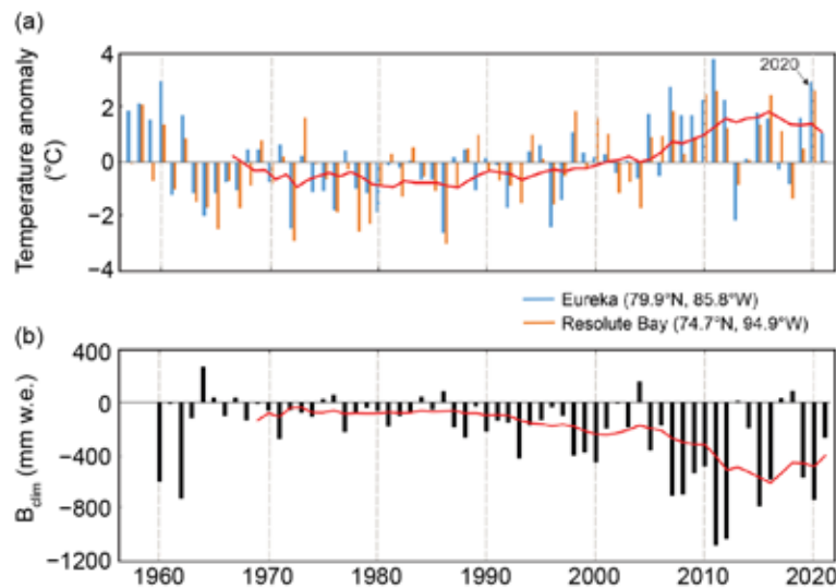
Fig. 5.17. (a) Annual temperature anomalies ( ^{\circ}\text{C} ) derived from the Integrated Global Radiosonde Archive (Imke et al. 2016) and (b) average climatic mass balance ( B_{clim} ; mm w.e.) for monitored glaciers in the Canadian High Arctic. Solid red lines indicate decadal averages. Summer temperature anomalies (JJA 850 hPa) and B_{clim} are strongly correlated with Pearson correlation coefficients of -0.8 and -0.97 for annual and decadal correlations, respectively, over approximately six decades for which overlapping measurements are available. Near-record high temperature anomalies in 2020 correspond to the fifth most negative B_{clim} measured since 1960.
