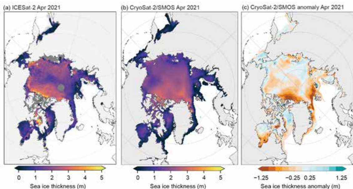
Fig. 5.9. (a) ICESat-2 (dark gray areas have no data) and (b) CryoSat-2/SMOS sea ice thickness (m) for Apr 2021; (c) CryoSat-2/SMOS thickness anomaly (m) for Apr 2021 (relative to the 2010–20 average). Note that ICESat-2 thickness estimates outside the Arctic Ocean domain (see the Fig. 5.8c inset) are not as reliable due to uncertainties in snow cover.
