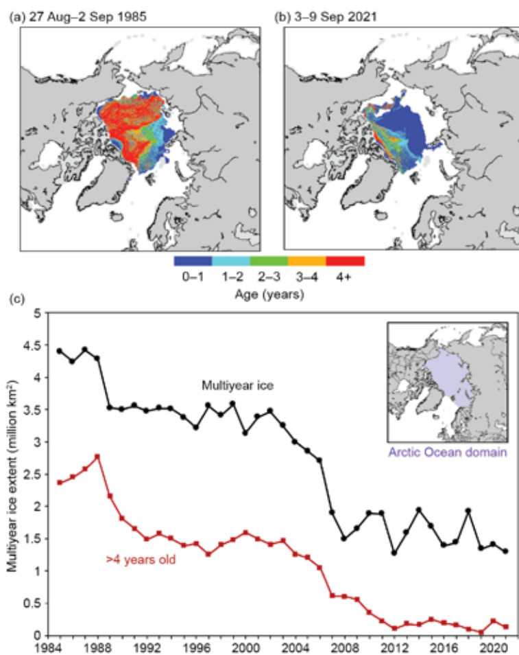
Fig. 5.8. Sea ice age coverage map for the week before minimum total extent (when age values are incremented to one year older) in (a) 1985 and (b) 2021; (c) extent of multiyear ice (black) and ice > 4 years old (red) within the Arctic Ocean (inset) for the week of the minimum total extent.
